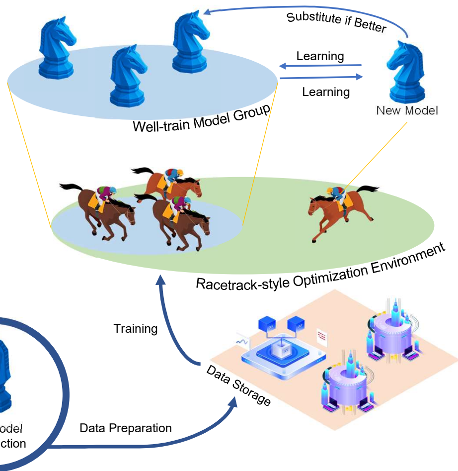
(b) Racetrack-style Optimization Strategy (Ours)
